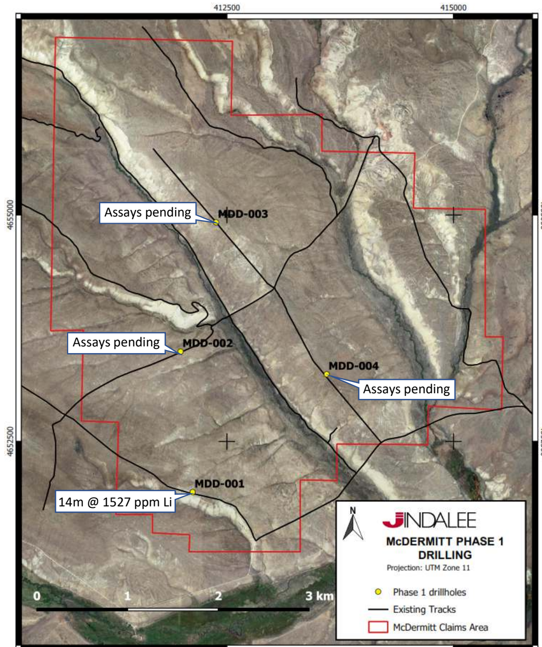
Figure 2 – Recently completed drill holes at McDermitt.
