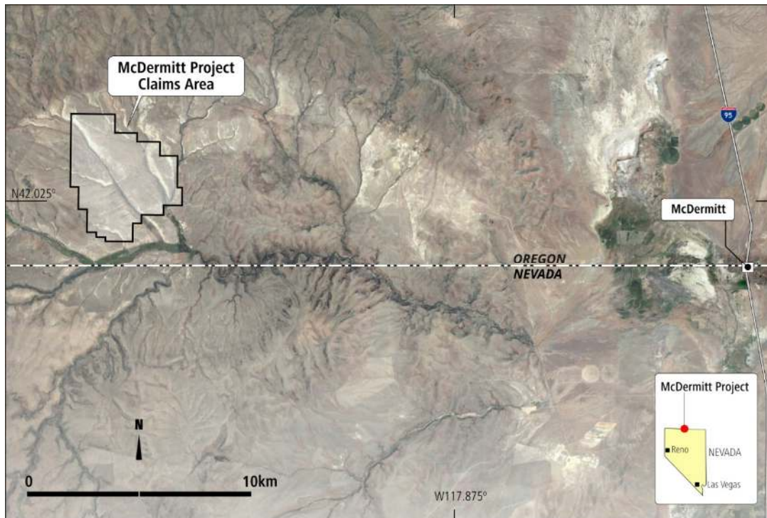
Figure 1 – Location of Jindalee's McDermitt Project
