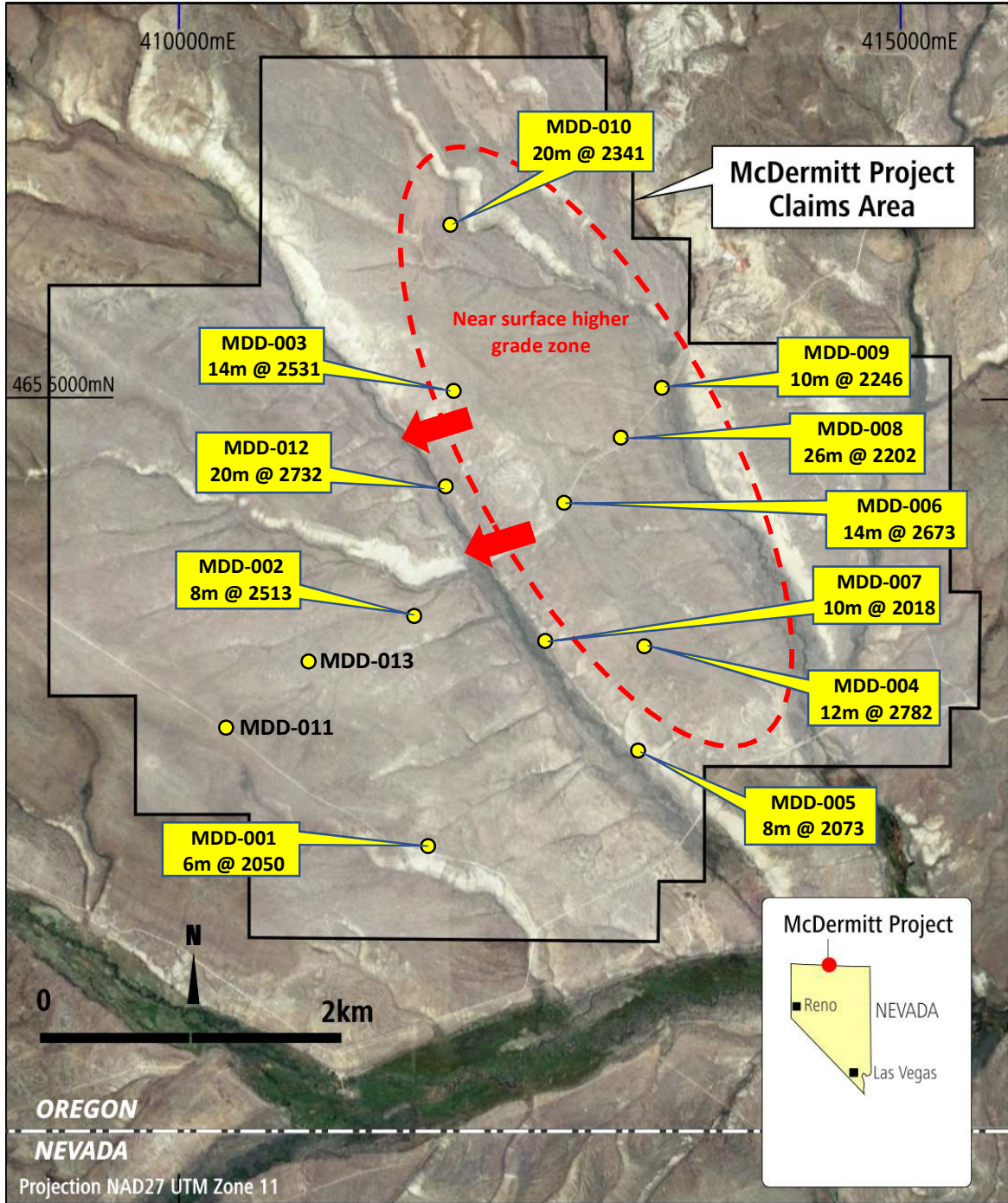
Figure 3 – Higher grade intercepts (Lithium ppm) at McDermitt highlighting the near-surface zone of higher-grade material >2200 ppm Li (red dashed oval) that can now be expanded westward based on the excellent results from MDD-012, and existing results from MDD-002.
