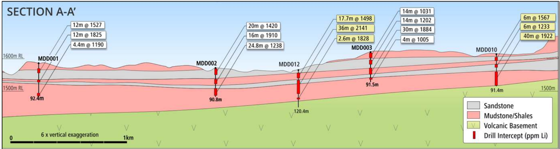
Figure 2 – Schematic cross section showing significant Lithium intercepts from the 2018 and 2019 drill programs.
