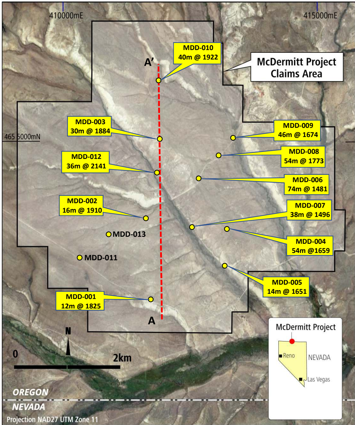
Figure 1 – Summary of the thick significant intercepts (Lithium ppm) so far received at McDermitt. Results from holes MDD-011 and 013 are awaited. The location of the cross-section A-A' in Figure 2 is shown as the red dashed line.
