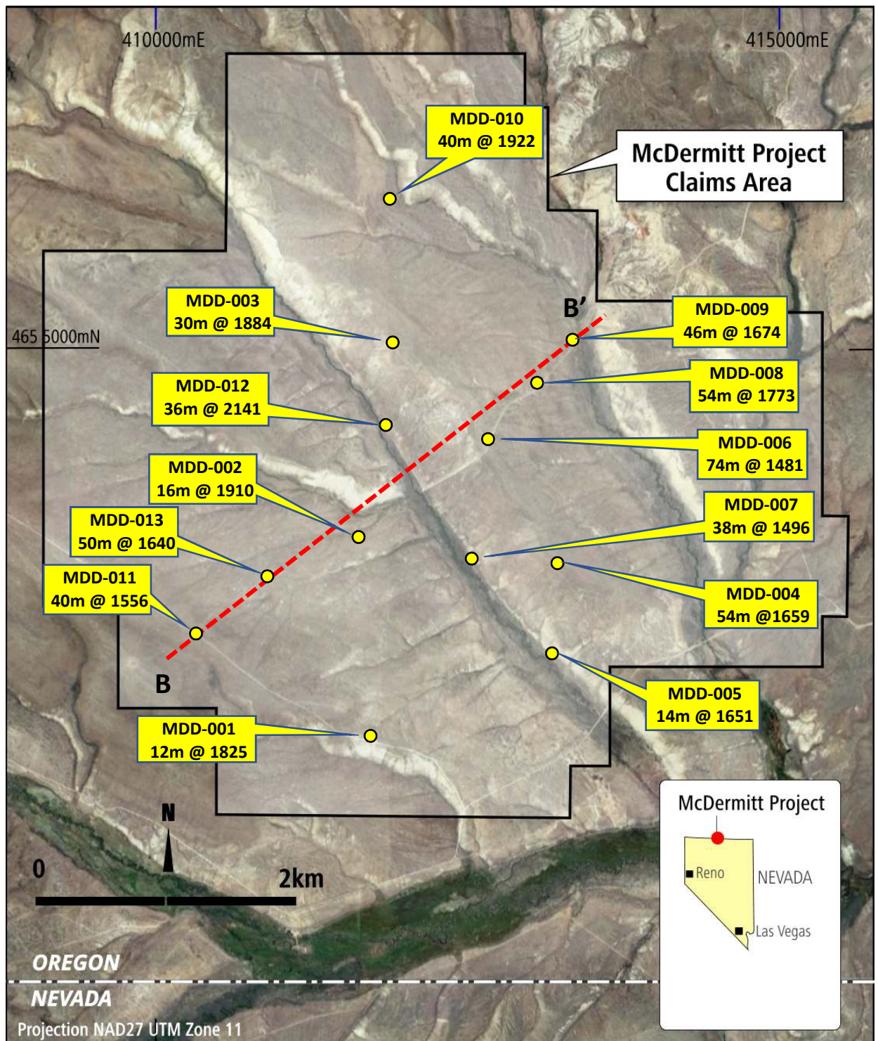
Figure 1 – Summary of the thicker significant intercepts (Lithium ppm) from drilling at McDermitt. The location of the cross-section B-B' in Figure 2 is shown as the red dashed line.
