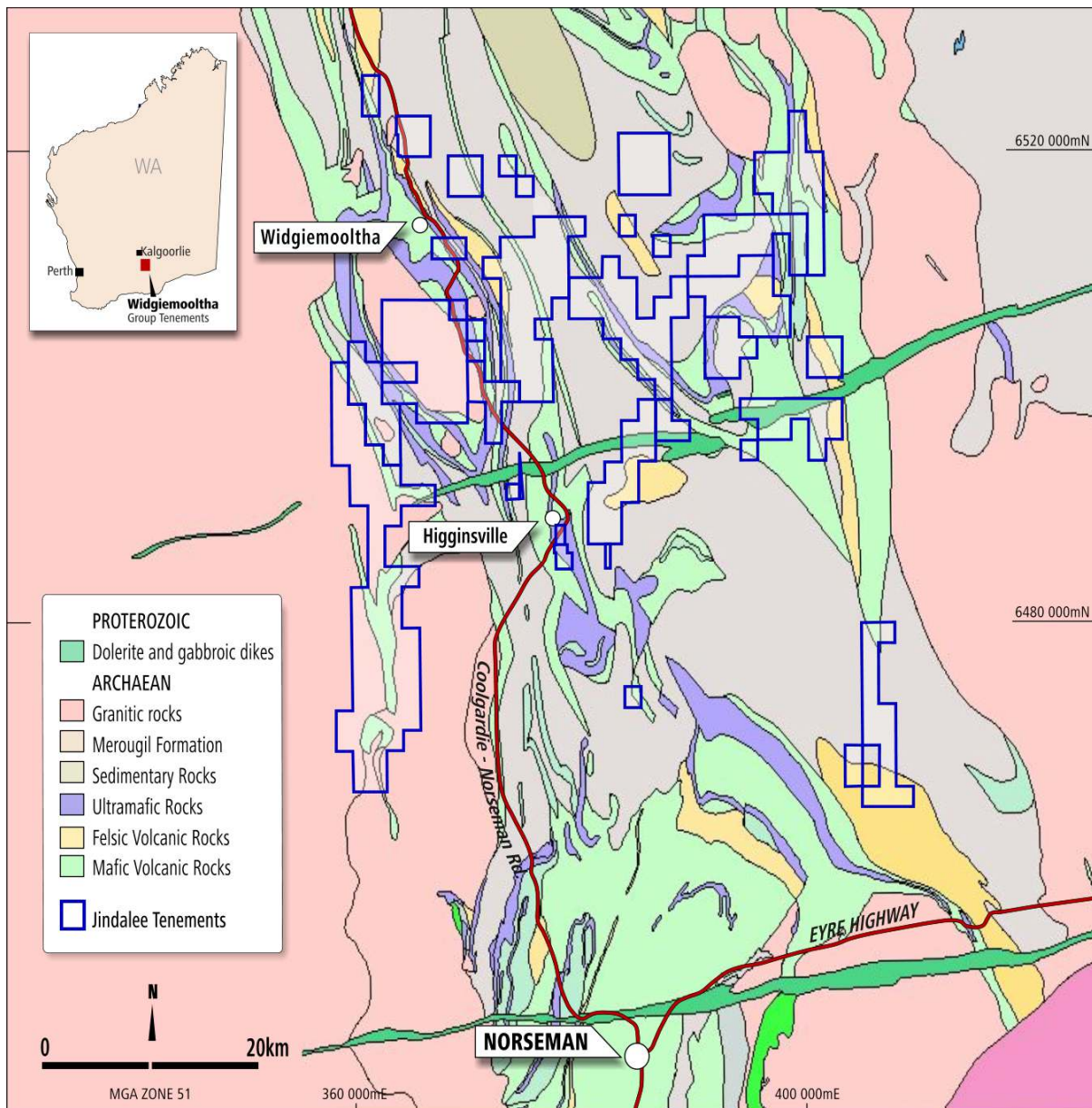
Figure 3: Widgiemooltha Project tenements (as at 30 June 2018) over regional geology. Note some portions of the tenements are excised by pre-existing mining and other leases.
